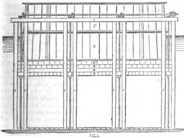
MODE OF SINKING PIERS AT SUSQUEHANNA BRIDGE.
